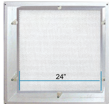
Comes Standard with 24" x 24" x 4" HEPA (MERV 13 Mini-Pleat avail.)
