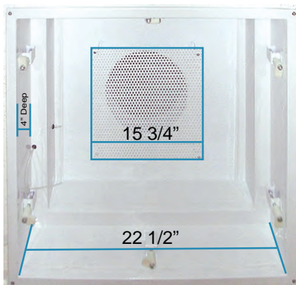
Inner Dimensions
